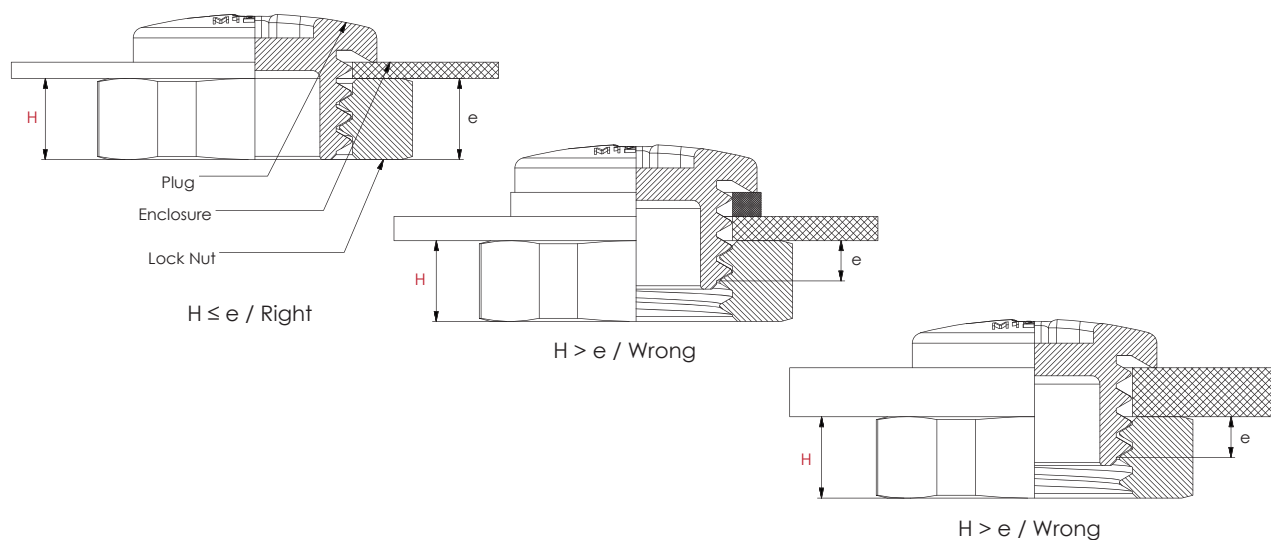
Relevant Lock Nut Thickness
